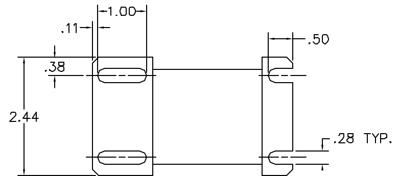
MOUNTING PLATE DETAIL
